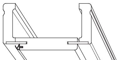
Zarge / Frame RP07
